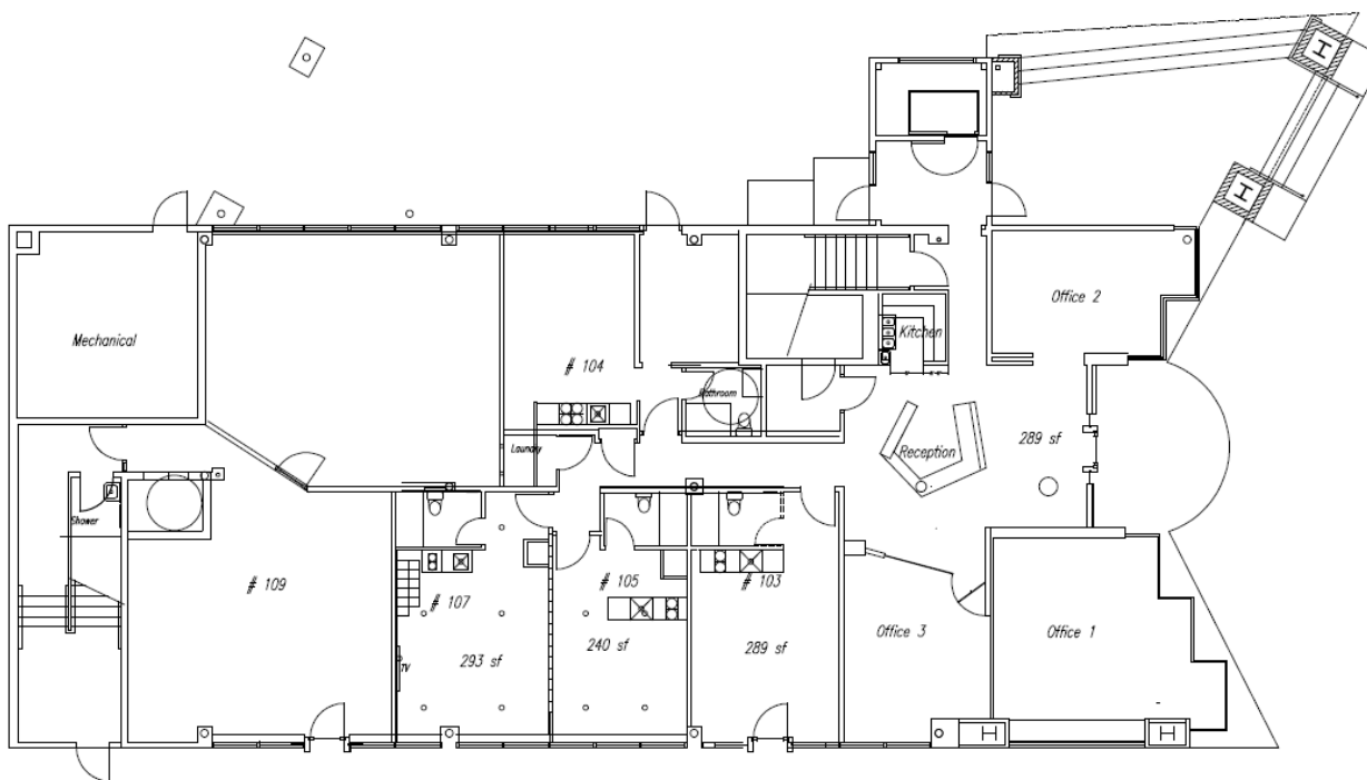
FIRST FLOOR 4100 SQFT
